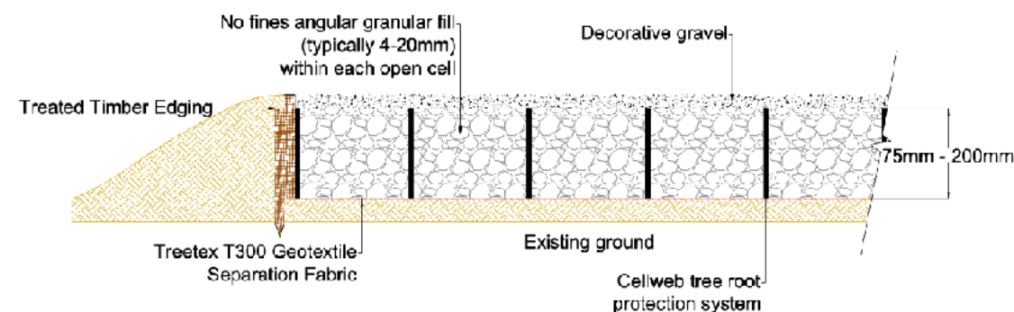
Figure 2: Typical Cellweb cellular confinement system cross-section.
